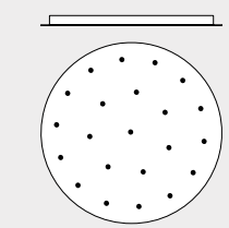
Ø900 mm [35.4"] 22 SUSPENSIONS 22 SOSPENSIONI
